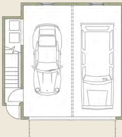
GARAGE LEVEL 24 SF
