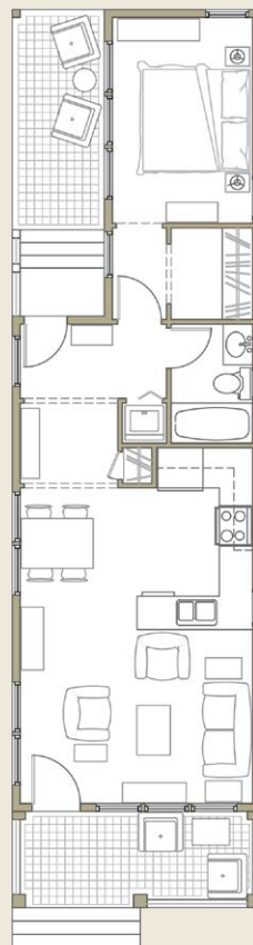
MAIN LEVEL 645 SF
