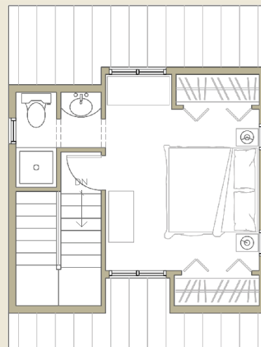
UPPER LEVEL 195 SF
