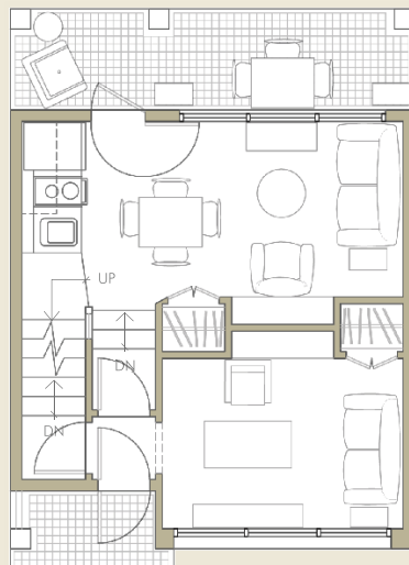
MAIN LEVEL 330 SF
