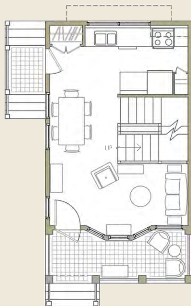
MAIN LEVEL 375 SF
