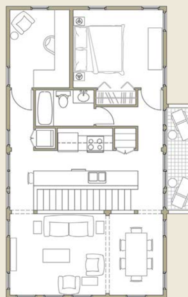
MAIN LEVEL 900 SF
