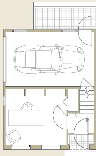
GARAGE LEVEL 335 SF
