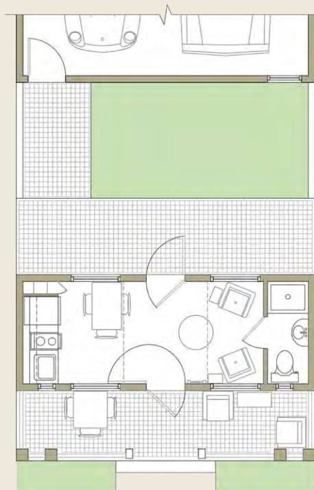
MAIN LEVEL 187 SF
