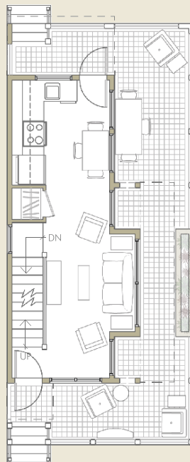
MAIN LEVEL 345 SF
