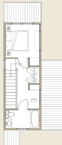
UPPER LEVEL 315 SF
