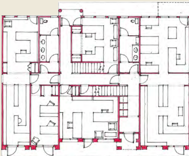
GROUND LEVEL 2,010 SF
