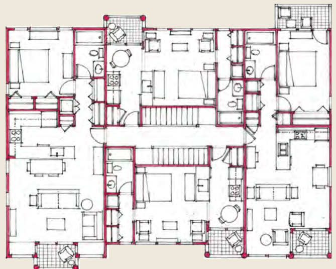
UPPER LEVELS 2,090 SF
