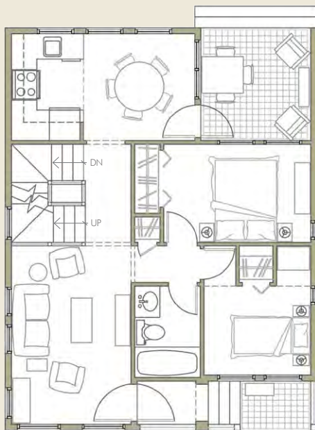
MAIN LEVEL 660 SF
